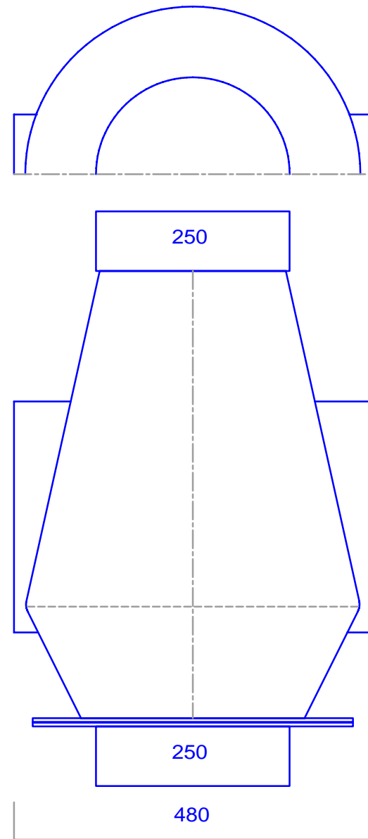
Calibre Plastics Ltd - Fumeflow Model TD250 In-Line Fan
