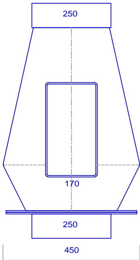
Calibre Plastics Ltd - Fumeflow Model TD250 In-Line Fan
